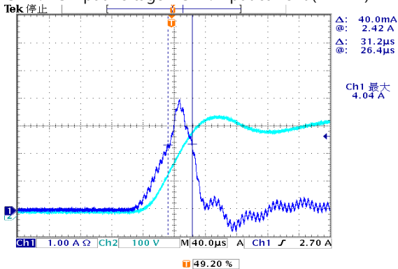
INPUT=230VAC/50HZ @ FULL LOAD
